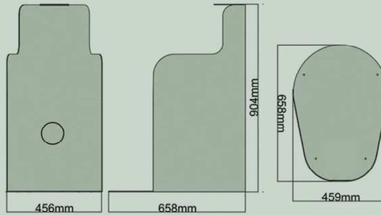
ApplePie Tall Enclosure
