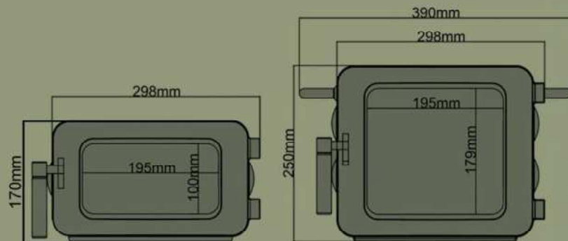
Removable Large Oven
